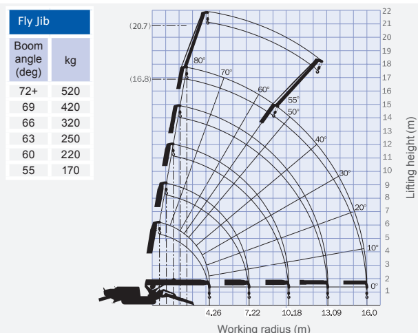
The Working Range Chart does not take into account boom deflection under load.
